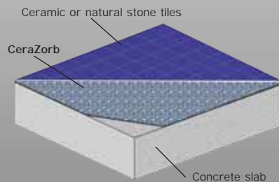
Typical Concrete Slab Construction
