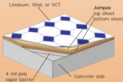
Typical Concrete Slab Construction
