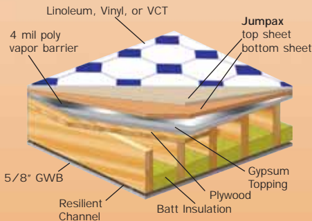
Typical Wood Construction
