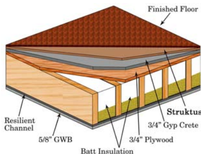
Typical Wood Construction
